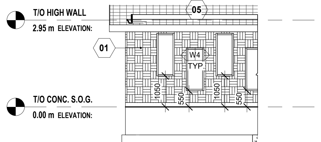
4 PARTIAL WEST 1 : 75
