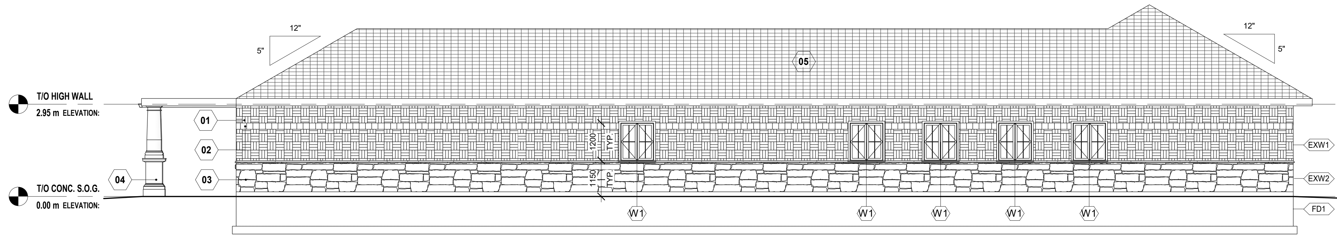
1 SOUTH 1 : 75
