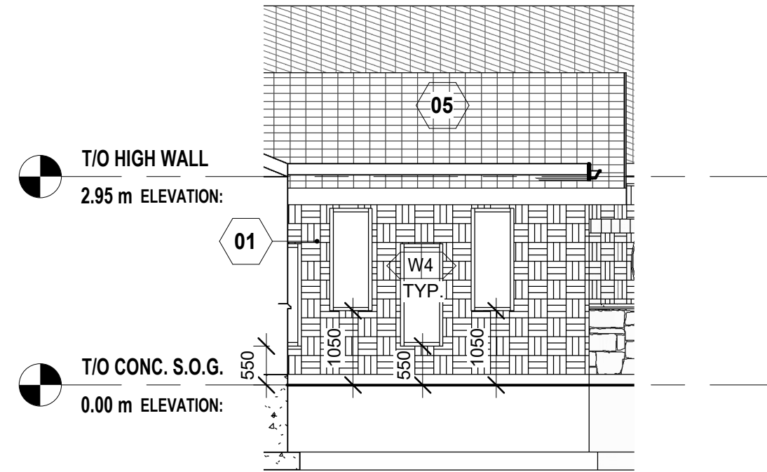
5 PARTIAL NORTH 1 : 75
